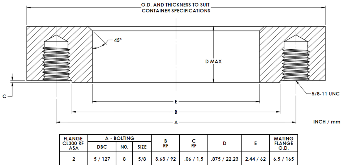
FIGURE 1: TANK FLANGE DIMENSIONS
